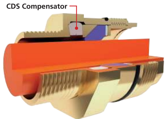
Figure 2 - When a larger diameter cable is installed the inner compensator operates to a greater extent.
